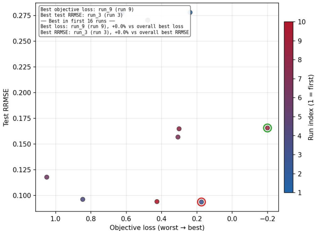
Loss vs Test RRMSE
